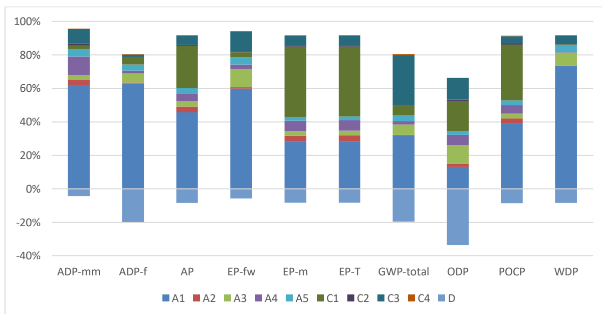
Figure 2: Tensar® TriAx® TX170 - Impact of the individual modules on the environmental core indicators (NMD set 2)
