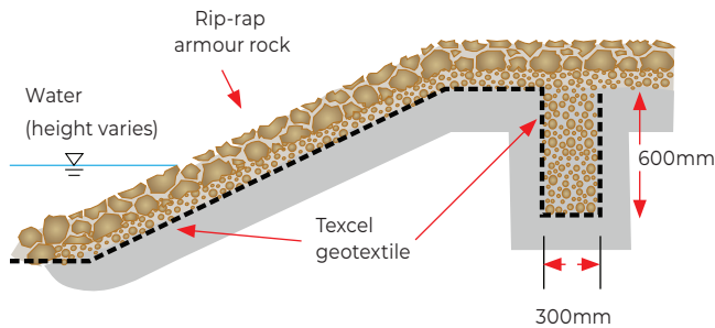
Figure 3. Revetments
